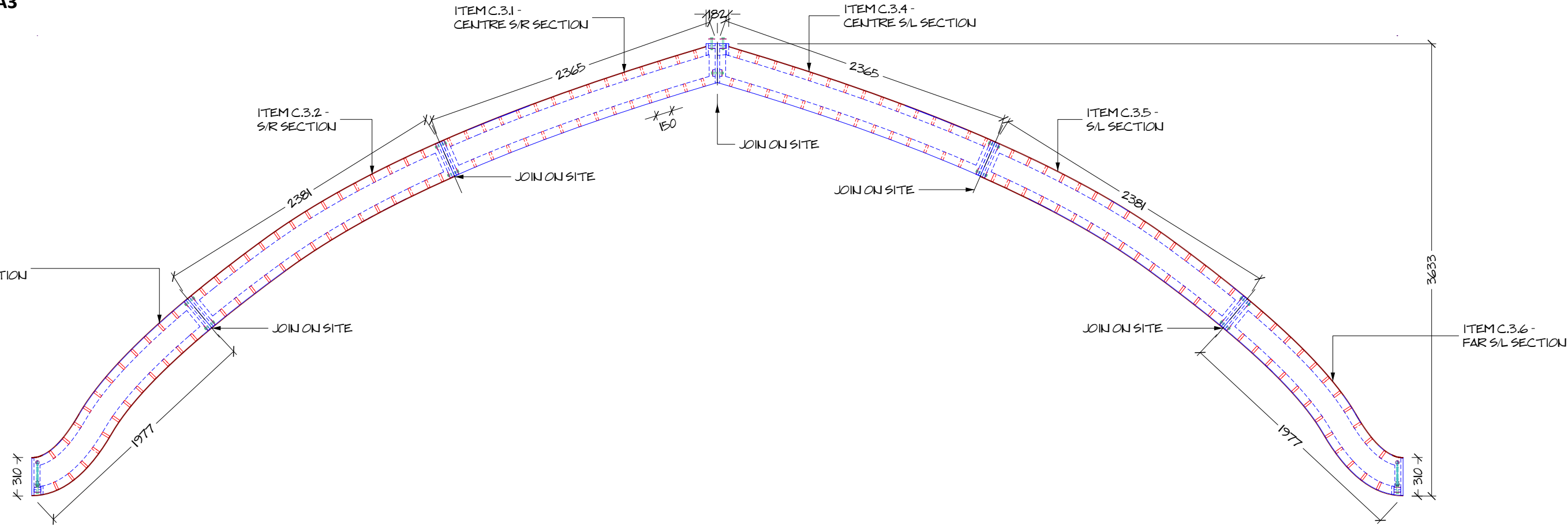
C.3 FRONT VIEW 1:35@A3
